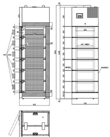
INDOOR/OUTDOOR - FROZEN 6 LOCKERS
