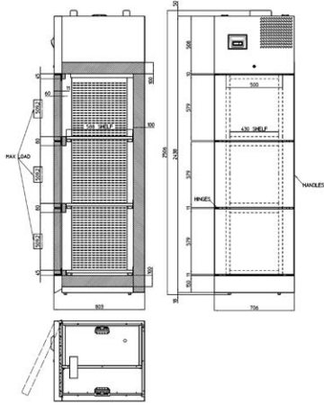
INDOOR/OUTDOOR - FRESH 3 LOCKERS OUTDOOR - DRY/AMBIENT 3 LOCKERS
