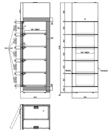
INDOOR - DRY 5 LOCKERS
