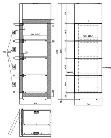
INDOOR - DRY 4 LOCKERS
