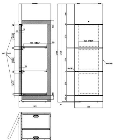
INDOOR - DRY 3 LOCKERS
